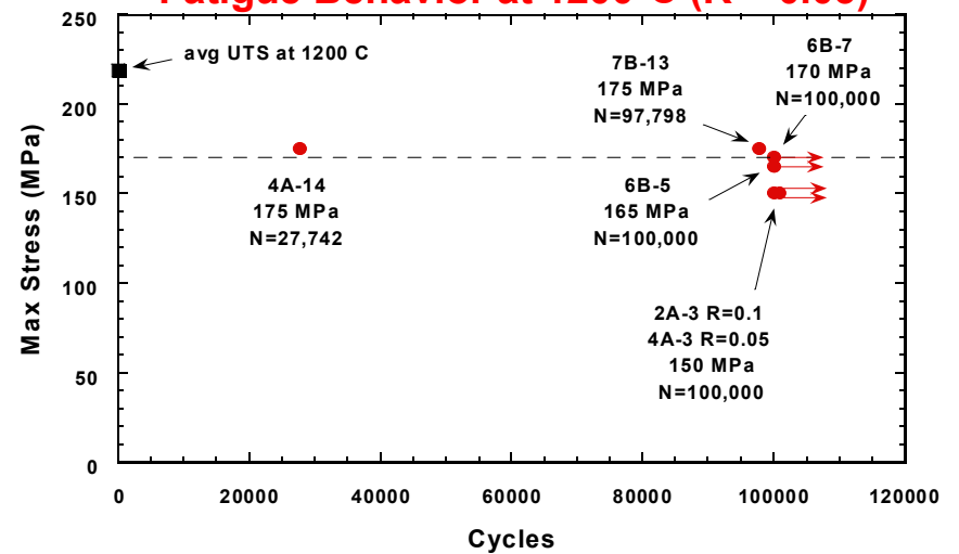
Fatigue Behavior at 1200°C (R = 0.05)
