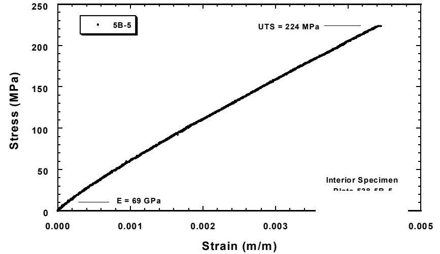
Tensile Strength at 1200°C
