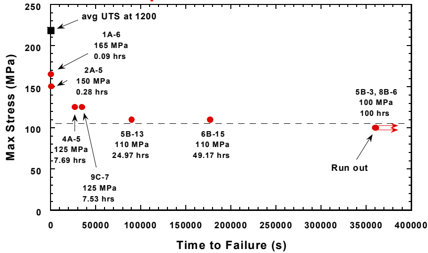
Creep Behavior at 1200°C
